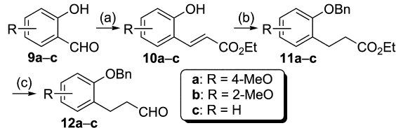
Scheme 2. Reagents and conditions: (a) \text{Ph}_3\text{P}=\text{CHCO}_2\text{Et} , \text{CH}_2\text{Cl}_2 , room temp., 1 h, 10a (96%), 10b (95%) and 10c (95%). (b) (i) \text{H}_2 , 10% Pd/C, EtOAc, 8 h, (ii) BnBr, anhyd. \text{K}_2\text{CO}_3 , dry acetone, reflux, 4 h, 11a (90%), 11b (87%) and 11c (91%) for combined two steps. (c) DIBAL-H, dry toluene, -78^\circ\text{C} , 1 h, 12a (95%), 12b (94%) and 12c (95%).
