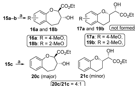
Scheme 4. Reagents and conditions: (a) (i) \text{H}_2 , 10% Pd/C, EtOAc, 8 h, 89%, (ii) anhyd. \text{K}_2\text{CO}_3 , dry acetone, room temp., 8 h, (iii) 20% \text{H}_2\text{SO}_4 , THF, room temp., overnight, 16a (70%), 18b (72%) and 20c (60%) and 21c (15%) for combined three steps.
